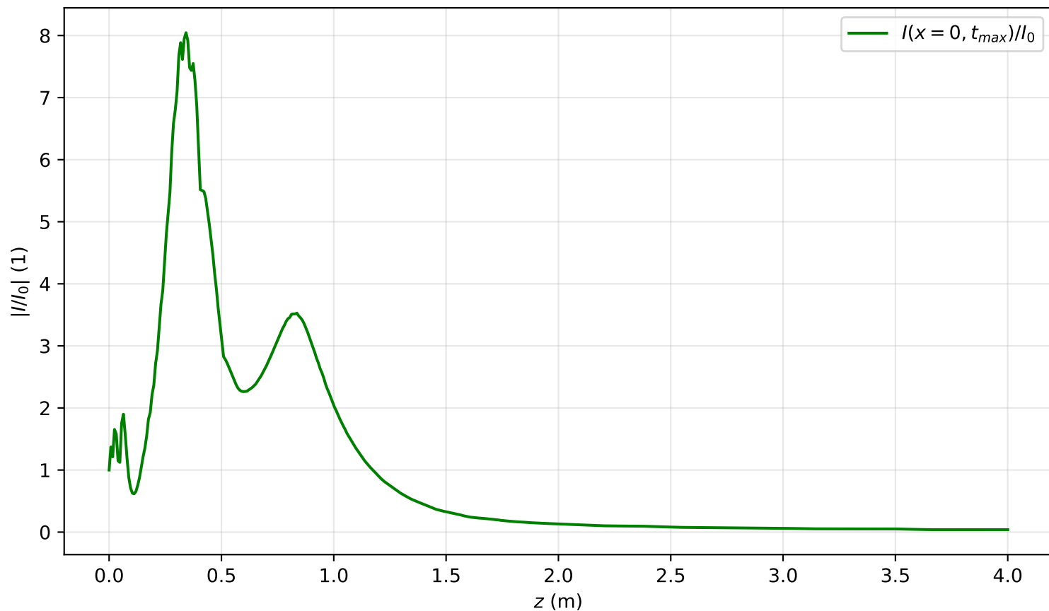
I(x=0, t_{max}, z)/I_0 , Pin=4.5Pcr
